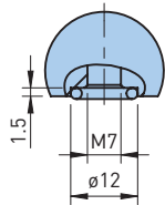
Detail A Scale 2:3 \phi 8 \times 2 O-Ring (Ships Plugged)
