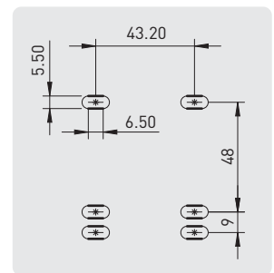
Mounting Bracket Positions
