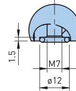
Detail B Scale 2:3 \phi 8 \times 2 O-Ring (Ships Plugged)
