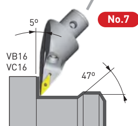
S50-SVLBR-33075-16 -SVLBL-33075-16
