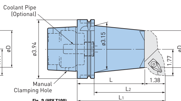
Fig. 2 (HSK-T100)
