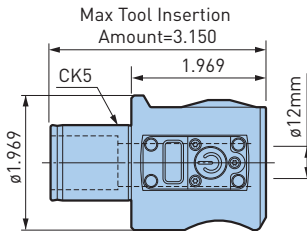
EWE2-32CK5 Stroke .020"-1.079"
