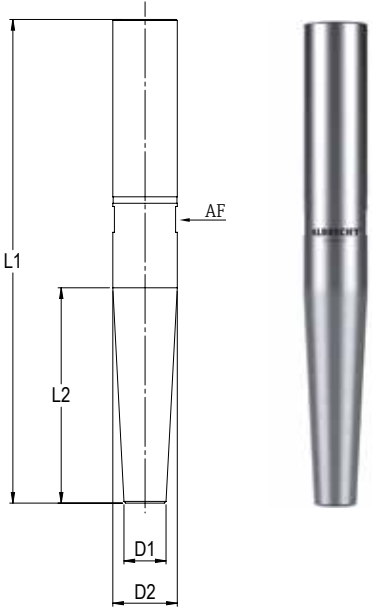
Cylindrical shank 20 mm 1 – 6 mm
