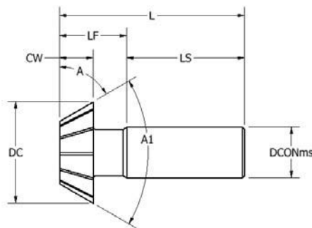
CH126 SINGLE-ANGLE
