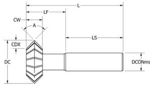
DA129 DOUBLE ANGLE
