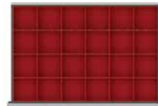
For drawer heights 75 through 125 PART NO. COMPTS. CMPT. WIDTH HWDR024-■ 24 6" x 6"
