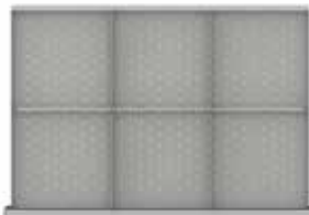
For drawer heights 75 through 200 PART NO. COMPTS. CMPT. WIDTH HWDR-LR106-■ 6 11.50"
